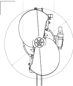
2 Blatt Propeller 2 Blades Propeller
