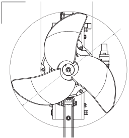
3 Blatt Propeller 3 Blades Propeller
