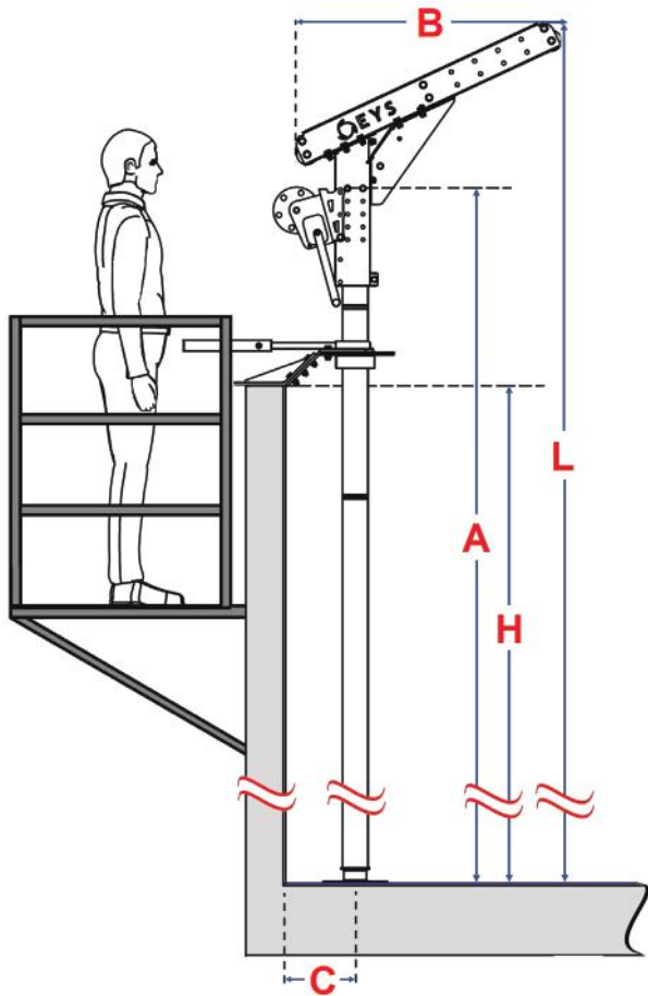
EYS Hebevorrichtung von DP Serie Pumpe Rotatable Platform – Lifting Devices
