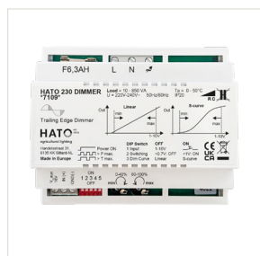
HATO 230 DIMMER (Phase dimming) *7109*
